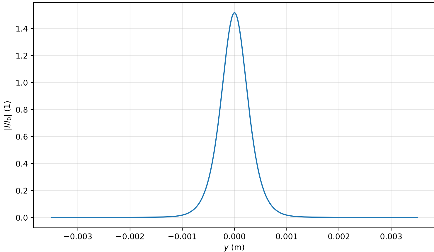
Intensity profile I(x=0, y, z=3.344)/I_0 , \text{Pin}=0.9\text{Pcr} , artificial time
